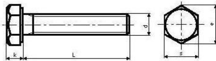
DIN933 Titanium Hexagon Head Screws
